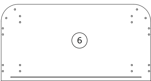
784x400x16 mm
